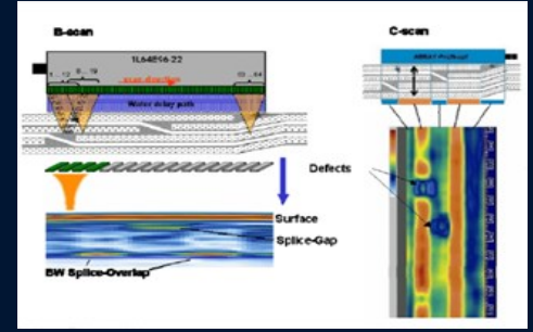
CB SCANNING TESTING
